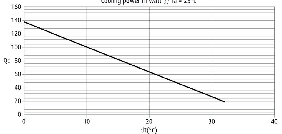
Performance graph Cooling power in Watt @ Ta = 25°C
