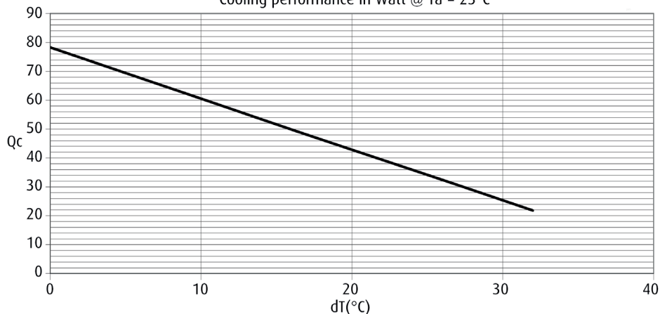
Performance graph Cooling performance in Watt @ Ta = 25°C
